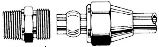
#99JM Tube Insert for J844A & J844B Metric Tube
